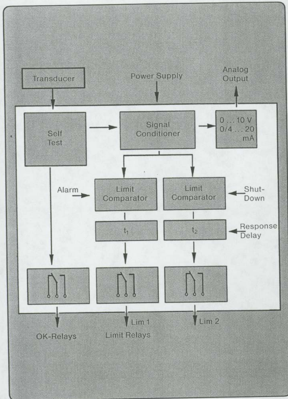
Fig. 3: Block diagram of VIBROCONTROL 1000 monitoring unit
