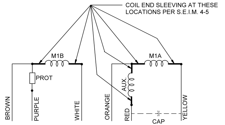
CONNECTION DIAGRAM
