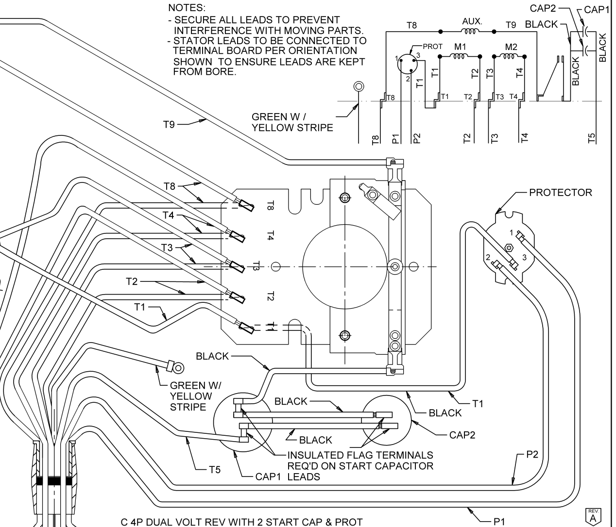
C 4P DUAL VOLT REV WITH 2 START CAP & PROT
