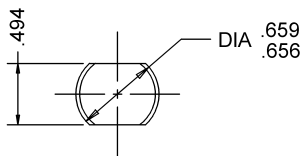
VIEW A-A (SHAFT GUARD NOT SHOWN FOR CLARITY) SCALE: 1/1
