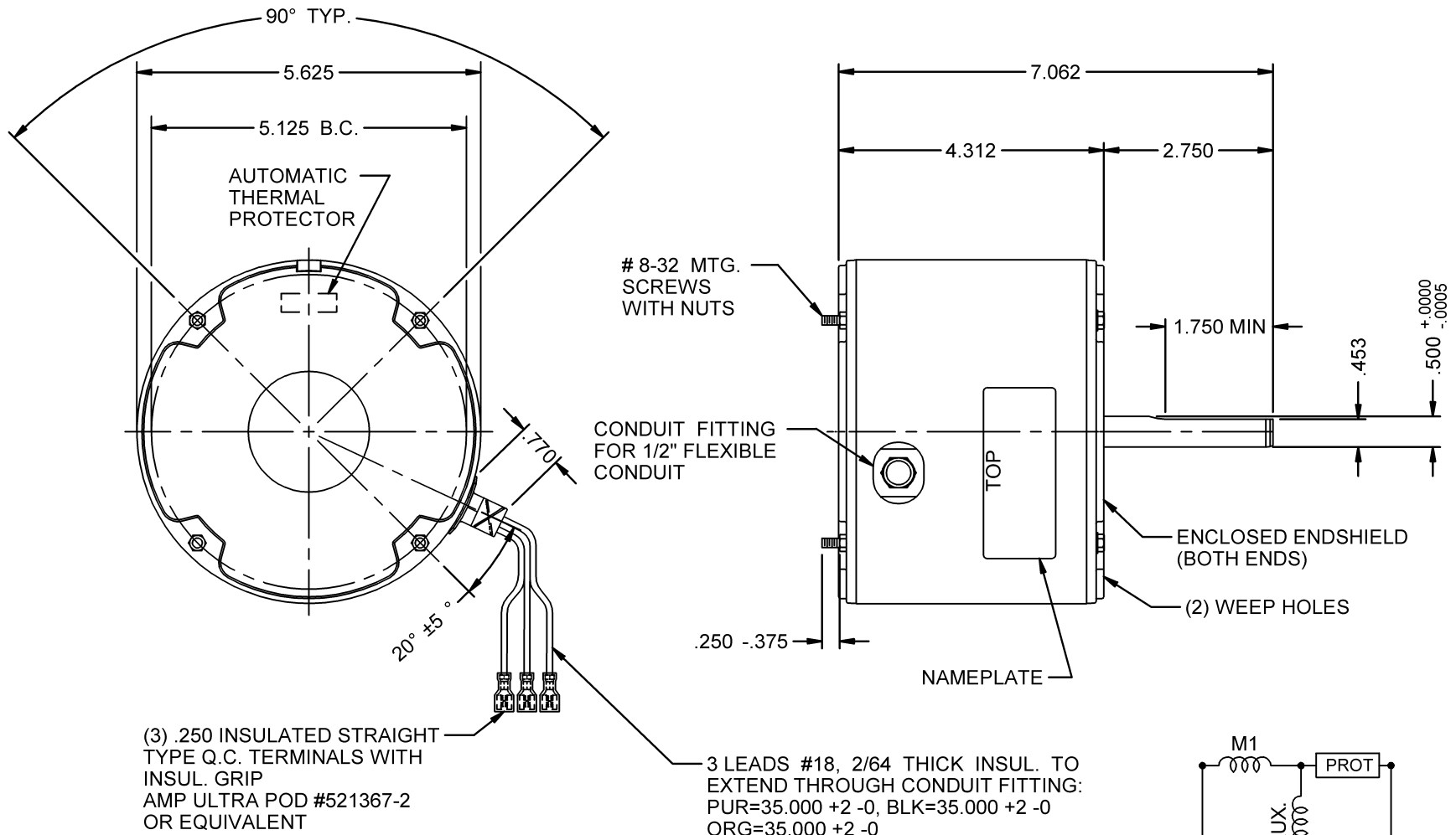
MOTOR MOUNTED IN SHAFT-DOWN POSITION
