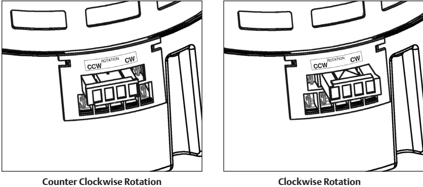
Figure 5 Note: Wire leads omitted for clarity.
