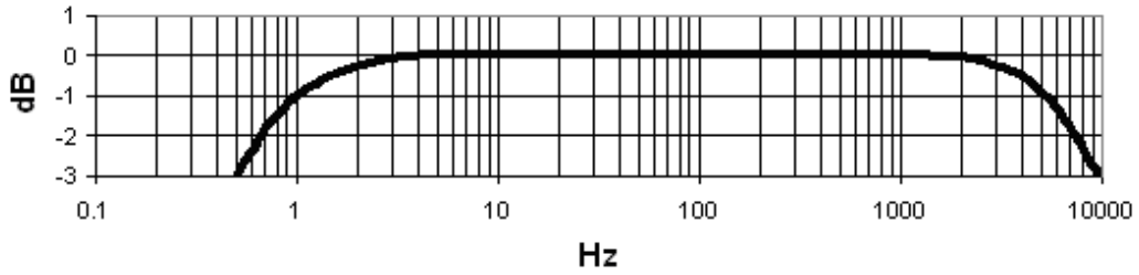
Figure 3. 200350 Accelerometer Frequency Response
