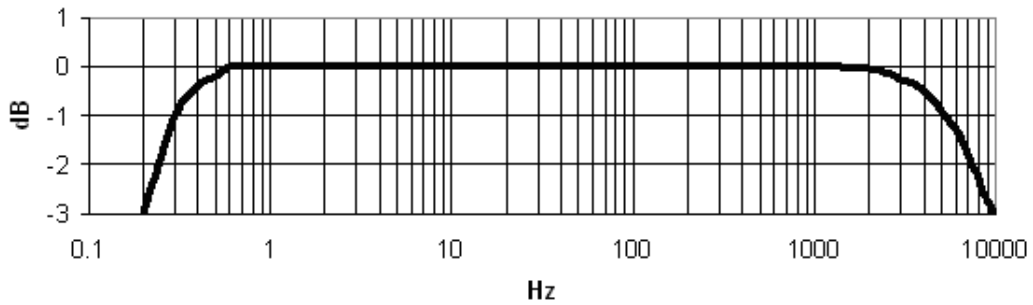
Figure 5. 200355 Accelerometer Frequency Response
