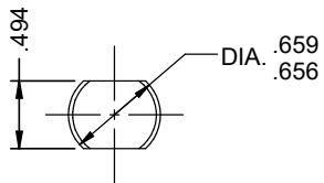
VIEW A-A (SHAFT GUARD NOT SHOWN FOR CLARITY) SCALE: 1/1
